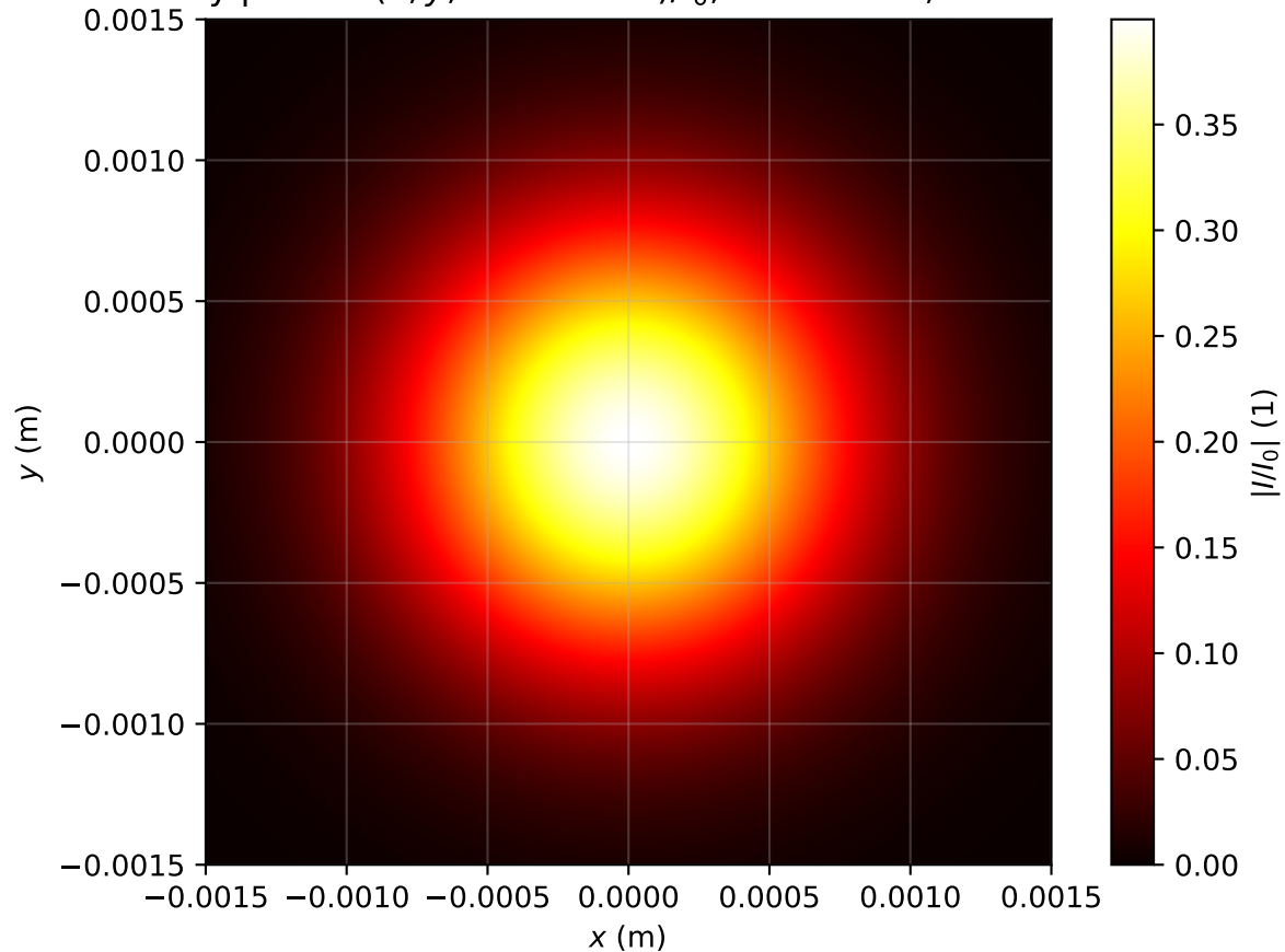
Intensity profile I(x, y, z = 2.627m)/I_0 , P_{in}=0.1P_{cr} , artificial time
